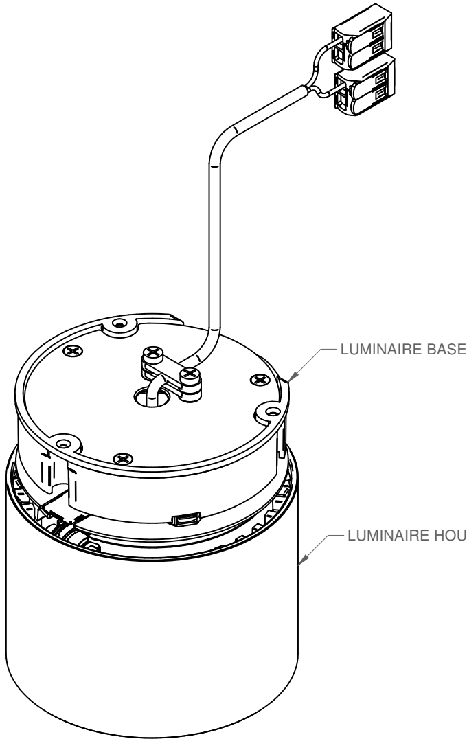
ISOMETRIC VIEW
