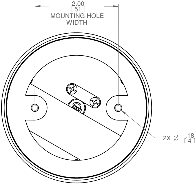
TOP VIEW 20MM CONDUIT JUNCTION BOX
