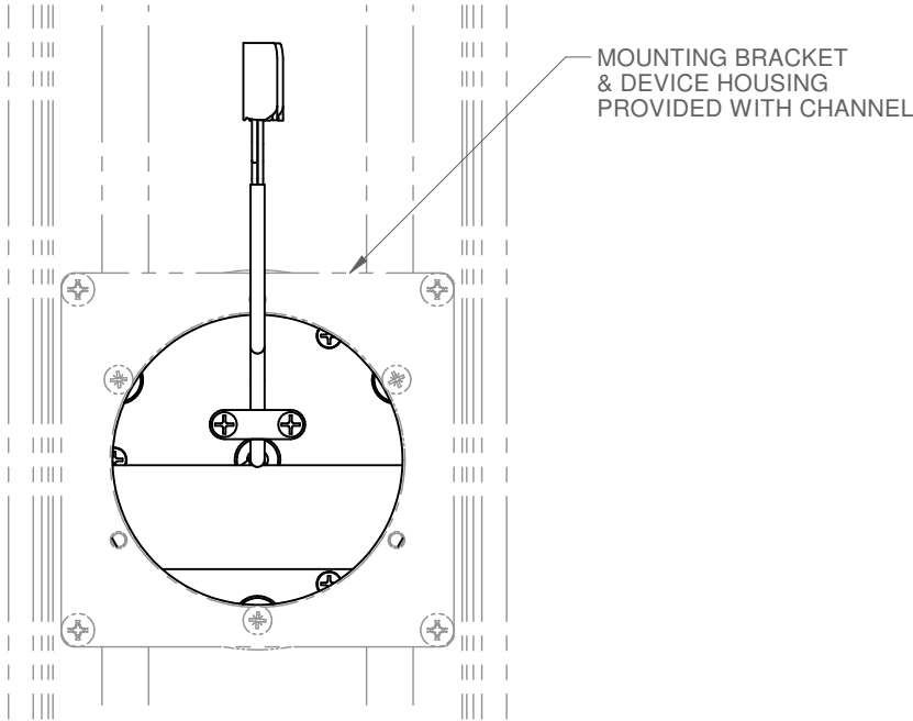
FLUSH CHANNEL TOP VIEW
