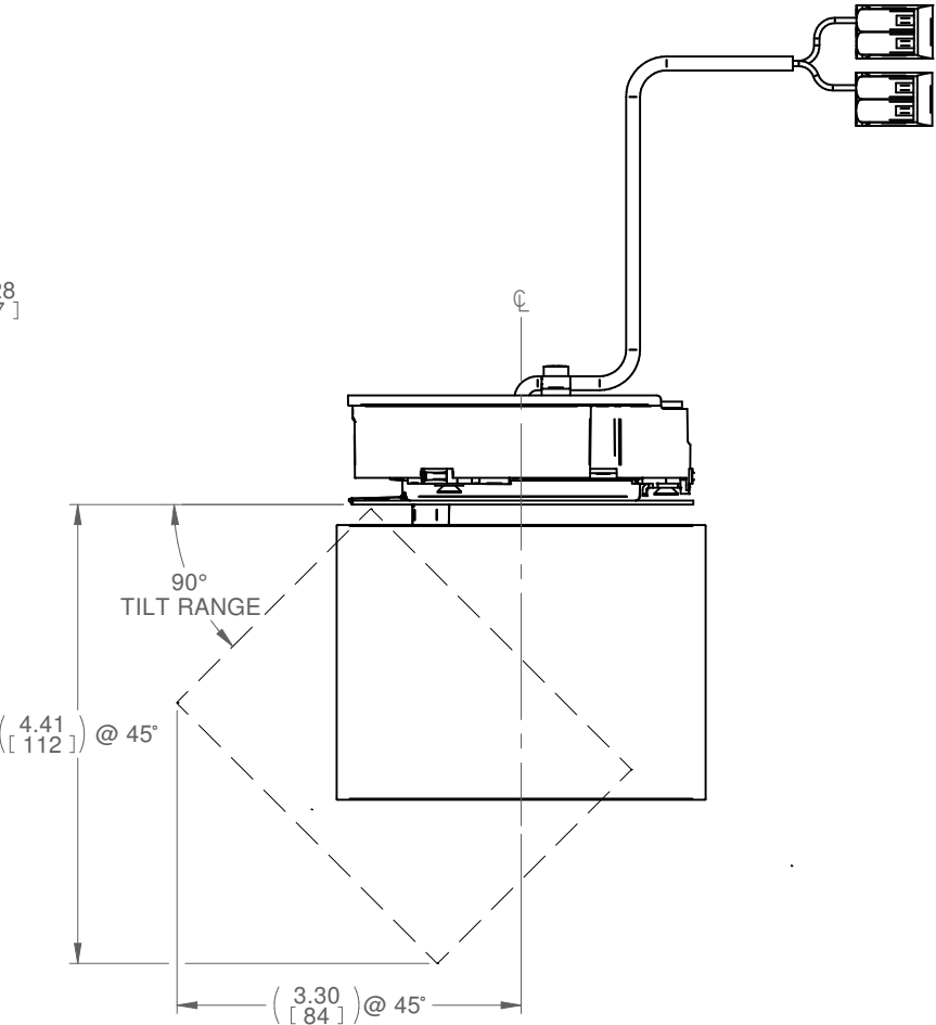
SIDE VIEW
