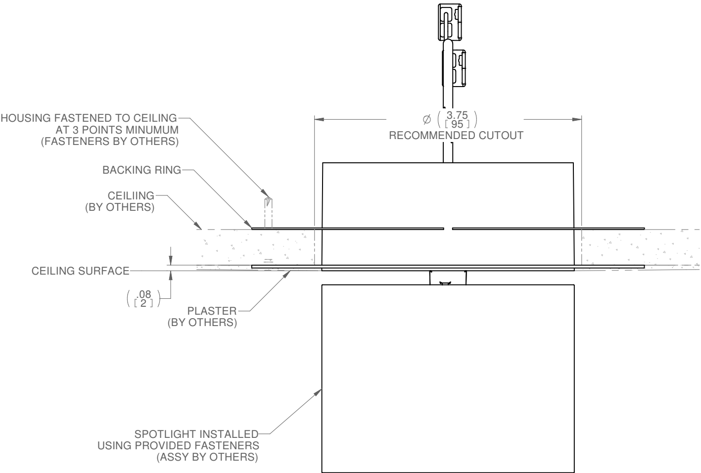
CEILING CROSS SECTION
