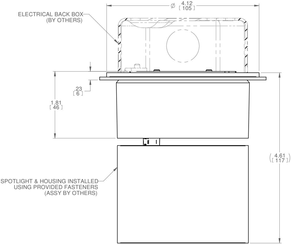
SIDE VIEW 4IN ROUND/OCT BOX
