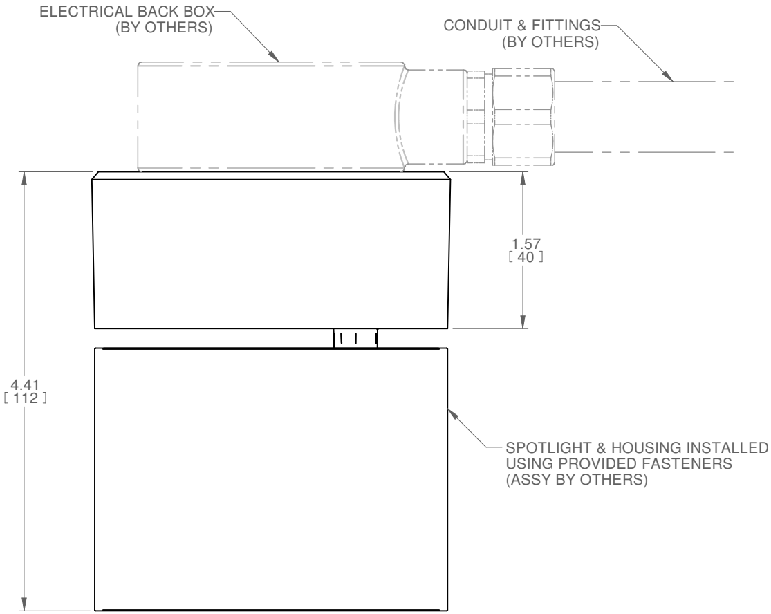
SIDE VIEW 20MM CONDUIT JUNCTION BOX
