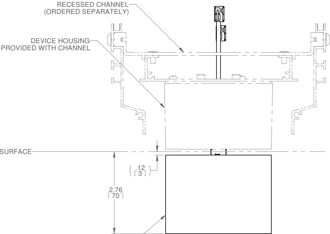
RECESSED CHANNEL END VIEW
